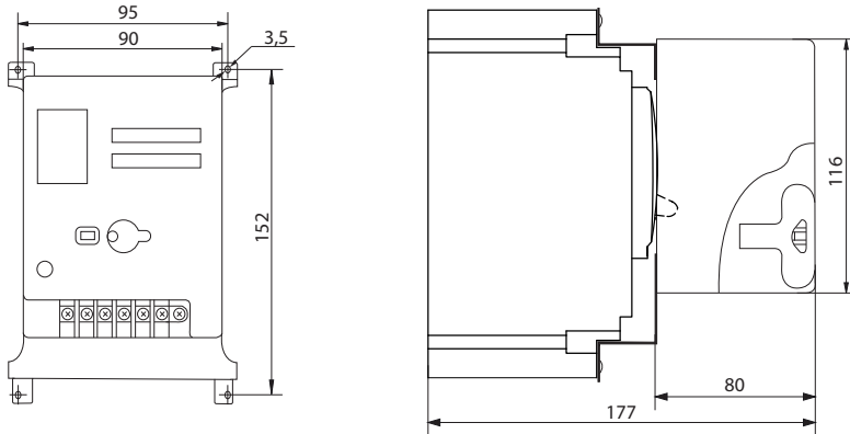
NBS-MO 400-630AF
