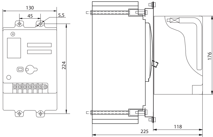
NBS-MO 400-630AF
